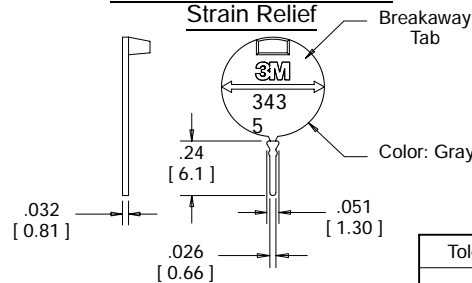
3435-0 Keying Plug
